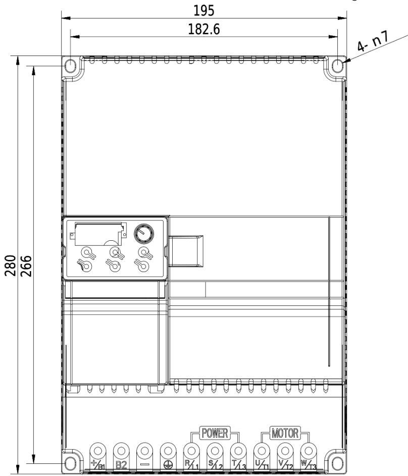
Dimensional drawing V800 - 15kW 4T0150
