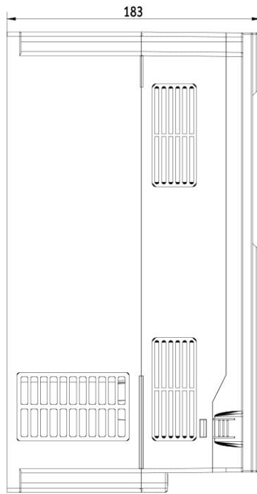
Dimensional drawing V900 - 30kW 4T0300
